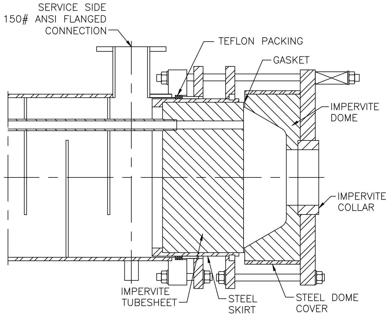
SKIRTED FLOATING TUBESHEET IMPERVITE SHELL/TUBE UNIT
